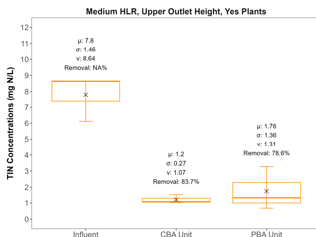
Figure 5. Box and whisker plot comparing effluent TIN concentrations for CBA and PBA operating at optimal configuration of medium HLR, upper outlet height, and Muhly Grass addition (after plant acclimatization).
