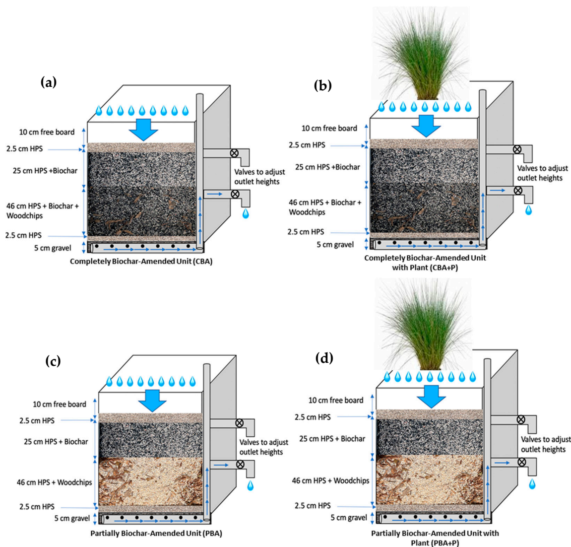
Figure 1. Schematic diagrams for the (a) completely biochar-amended (CBA) unit, (b) completely biochar-amended unit with plants (CBA + P), (c) partially biochar-amended (PBA) unit, and (d) partially biochar-amended unit with plants (PBA + P).
