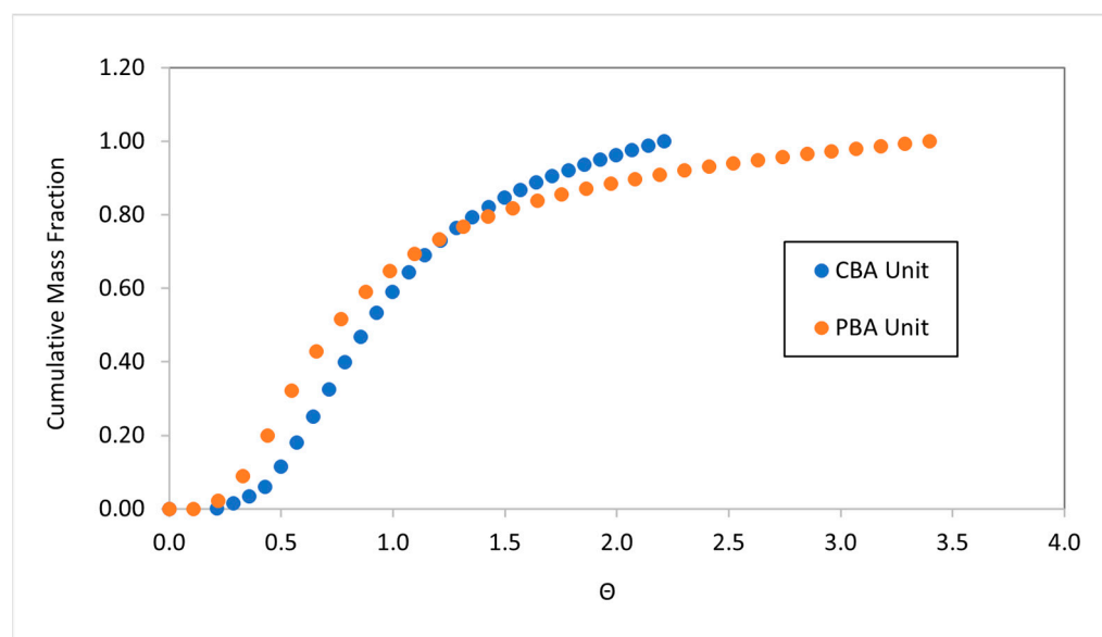
Figure 2. Cumulative tracer mass fraction exported vs. \Theta for bioretention systems configured at their lower outlets.
