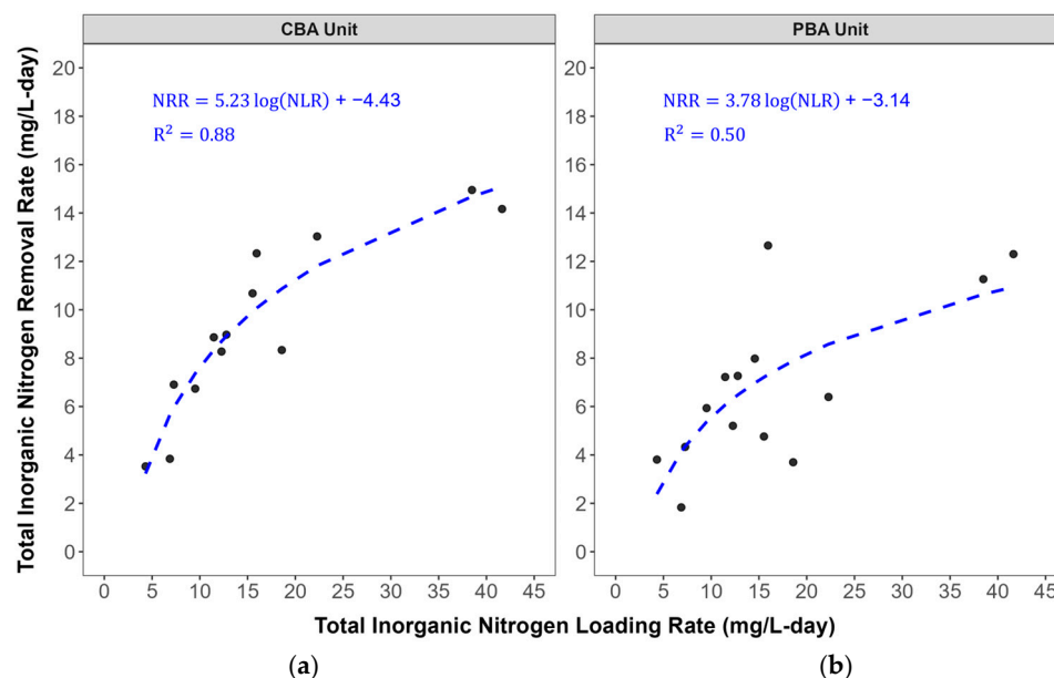
Figure 7. Logarithmic regression model for total inorganic nitrogen removal for the (a) CBA unit and (b) PBA unit.
