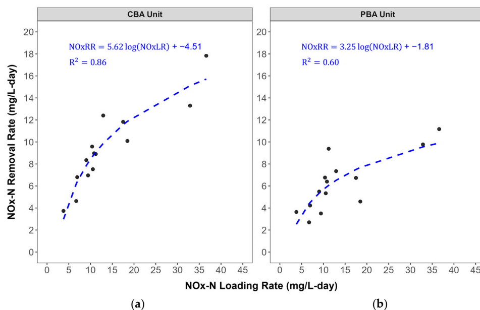
Figure 8. Logarithmic regression model for nitrate + nitrite (NO x ) removal for the (a) CBA unit and (b) PBA unit.
