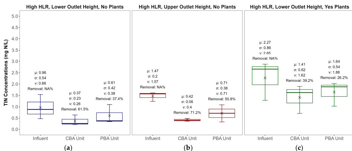
Figure 4. Box and whisker plots comparing effluent TIN concentrations for CBA and PBA units across varying outlet height (IWSZ depth). Figure (a,b) are without plant amendment. Figure (c) is with plant amendment. A comparison of Figure (a,c) allows an assessment of the effects of Muhly Grass on TIN removal.
