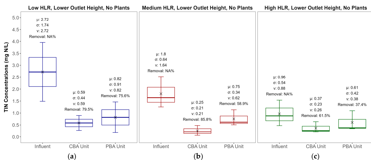
Figure 3. Box and whisker plots comparing effluent TIN concentrations for CBA and PBA units across varying HLR: (a) low, (b) medium, and (c) high.
